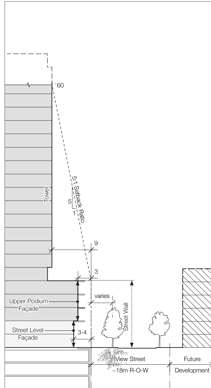
Non-prescriptive illustrative example. See Note 1 on page 6. Note this section illustrates the building form of both the 900-block and 1045 Yates.
