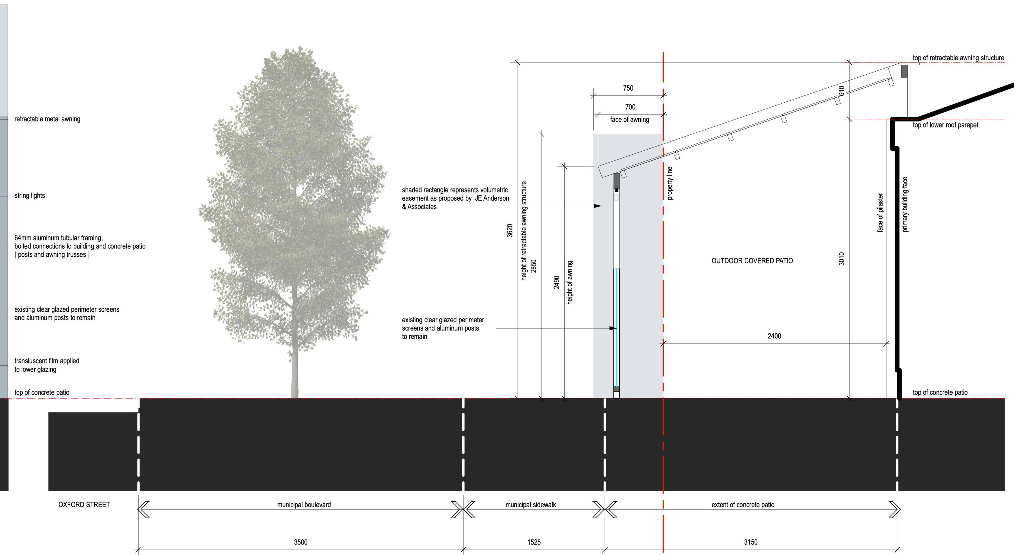
2 ROOF CANOPY CROSS SECTION A2.2 metric scale: 1 : 25
