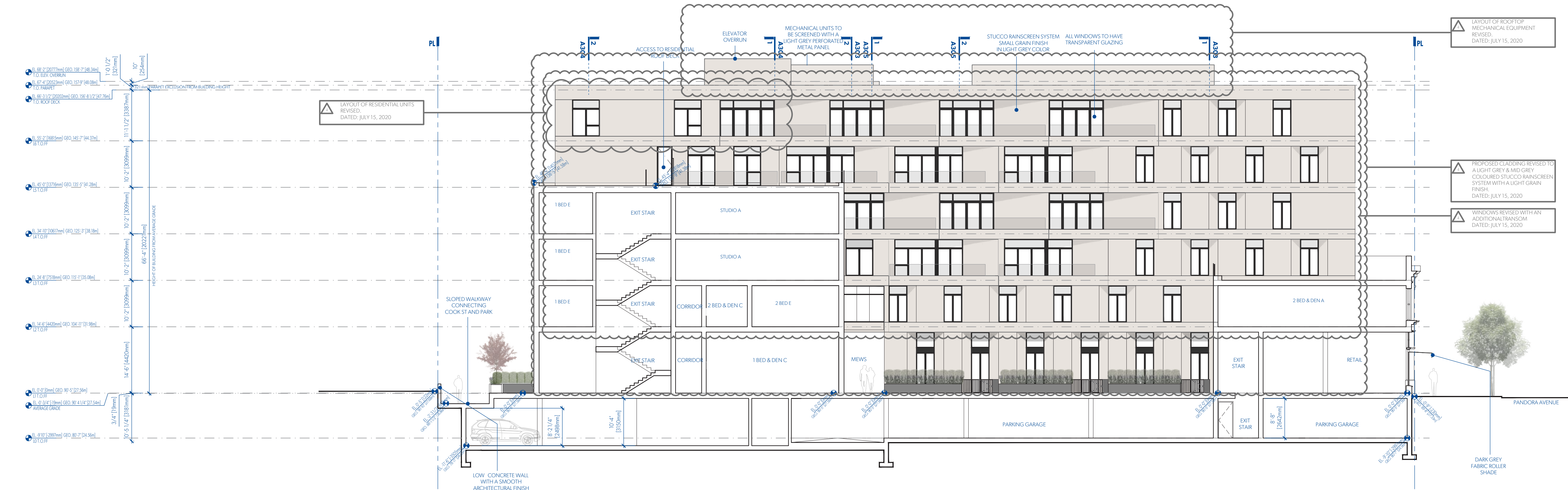
2 SECTION LOOKING EAST THROUGH NEW 4 STOREY VOLUME & EXISTING BUILDING A302 1:150
