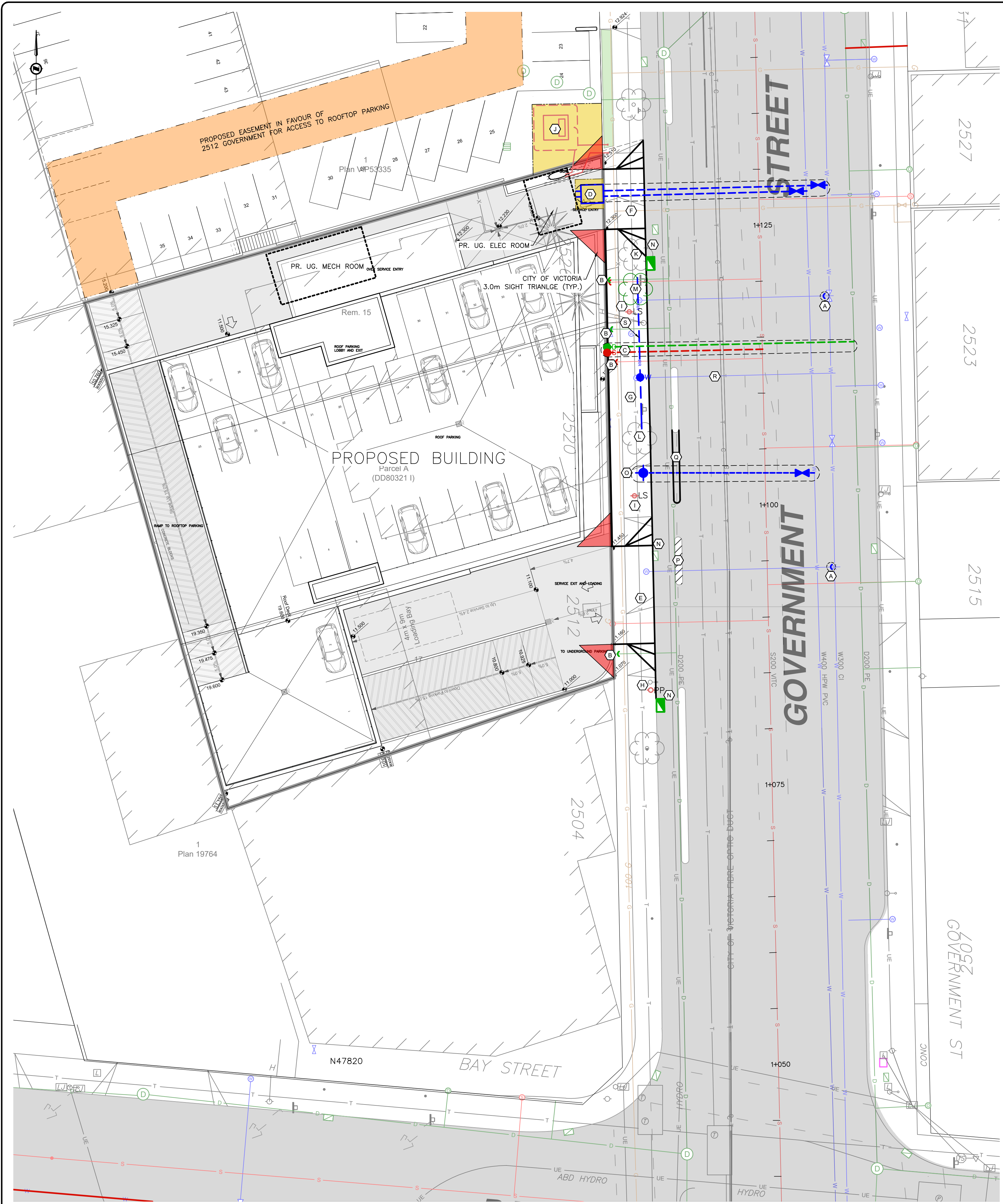
SITE SERVICING PLAN 1:200
